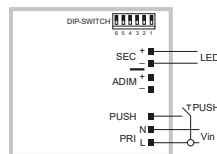
PUSH wiring diagram
