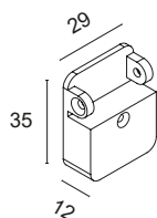
Fixing base
